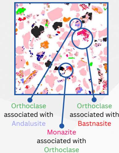
Pre-HPSA sample showing REE association in Orthoclase
