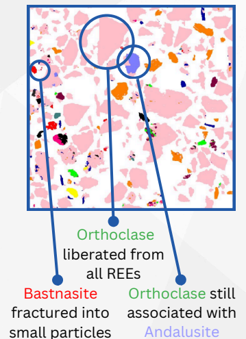
Post-HPSA sample illustrating fracture of REEs from hosted Orthoclase
